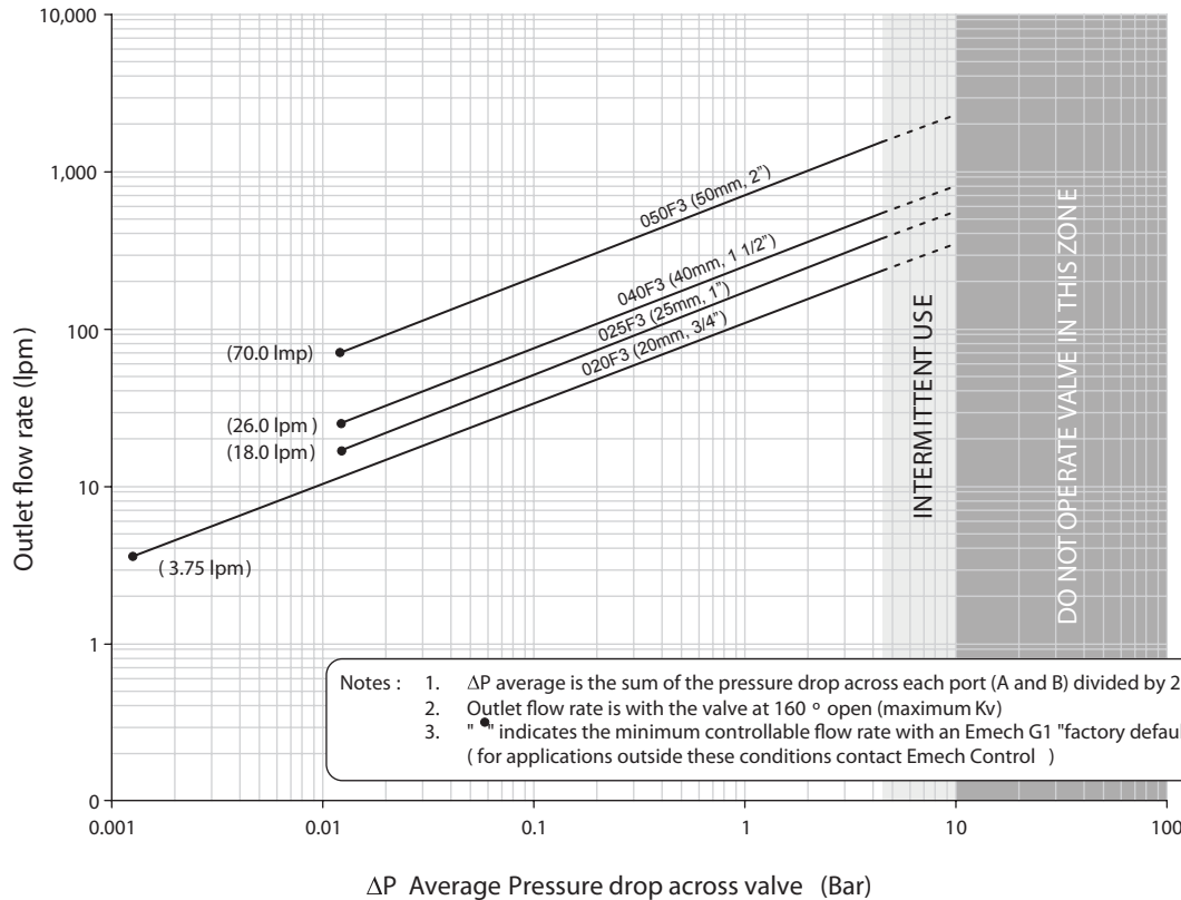
F3 Flow chart
