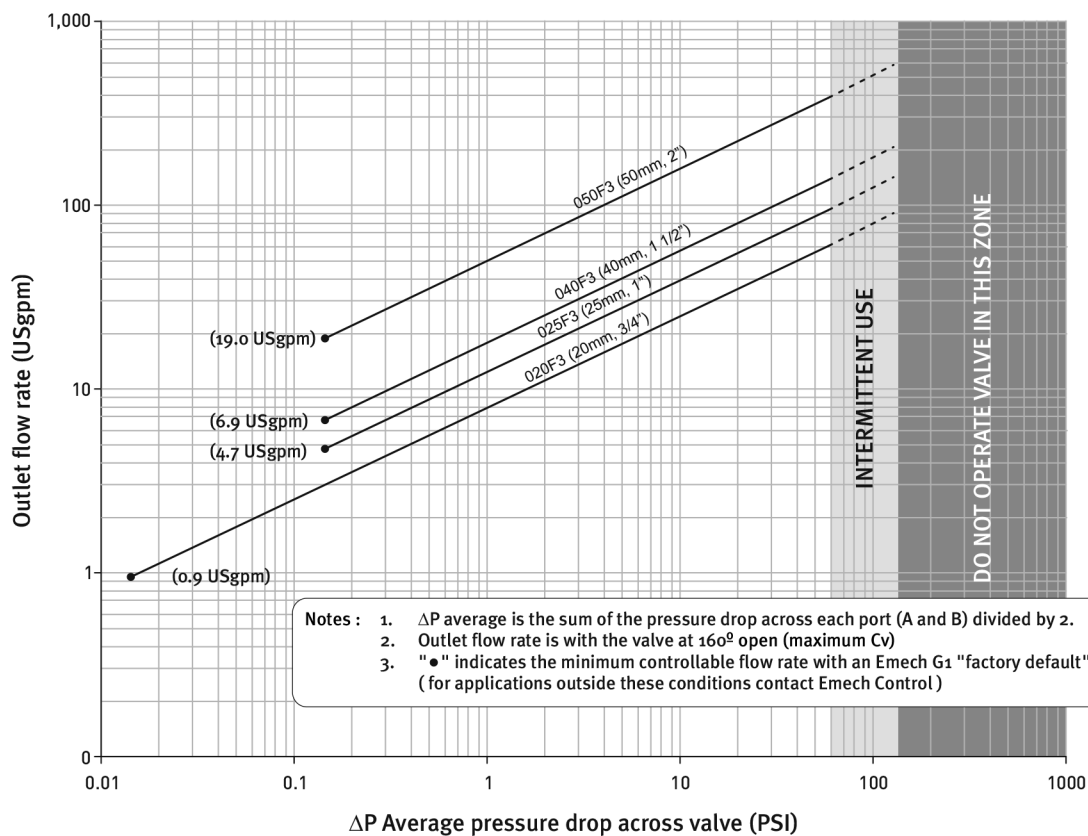
US flowrate co-efficients - Cv values
