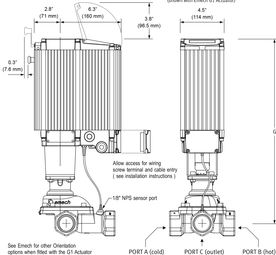
Emech F3 Valve (shown with Emech G1 Actuator)
